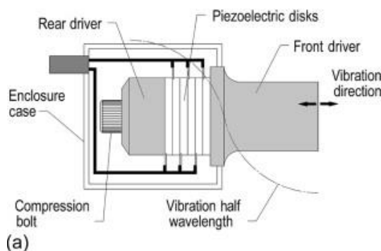
Above ultrasonic welding transducer
