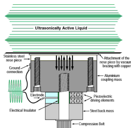
Above ultrasonic cleaning transducer
