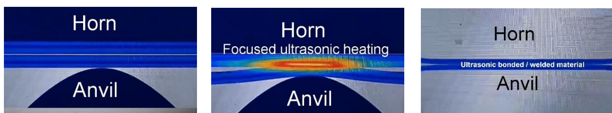
Thermographic illustration of temperature increases during welding
